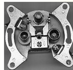
Triplexer with single input cable SMATV
