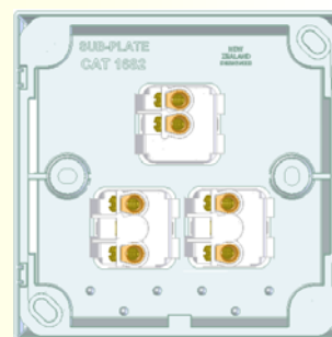
Rear View of 1683HA
