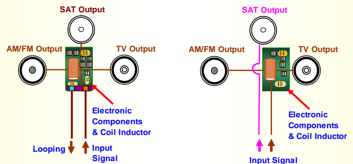
Satellite Master TV Antenna (MATV-1) Outlet with single input cable & looping facility
