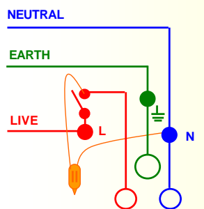
1667LN 1 Gang Single Pole Socket
