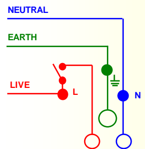
1667L 1 Gang Single Pole Socket
