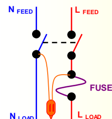
Fused Connection Unit 1626LN with Neon
