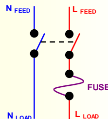
Fused Connection Unit 1626L
