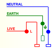
1660 1 Gang Single Pole Unswitched Socket
