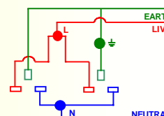
1668 2 Gang Single Pole Unswitched Socket
