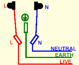
1679 1 Gang Hybrid Socket
