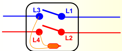
Rear view of CAT 1520N 1 Way Single Pole Plate Switch with neon indicator
