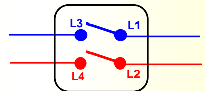
Rear view of CAT 1520 1 Way Single Pole Plate Switch
