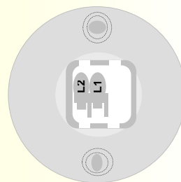
Rear view of 1573 1 Way Single Pole Switch Plate
