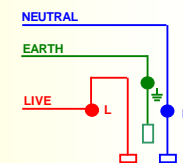
1560 1 Gang Single Pole Unswitched Socket
