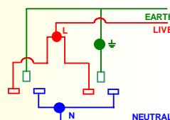
1568 2 Gang Single Pole Unswitched Socket
