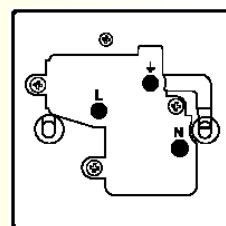
Rear View of CAT 1564 1 Gang Single Pole Socket
