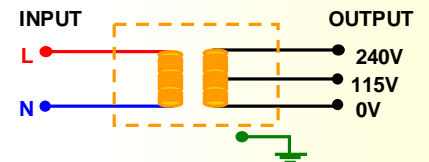
Circuit Diagram for 1575 Shaver Socket
