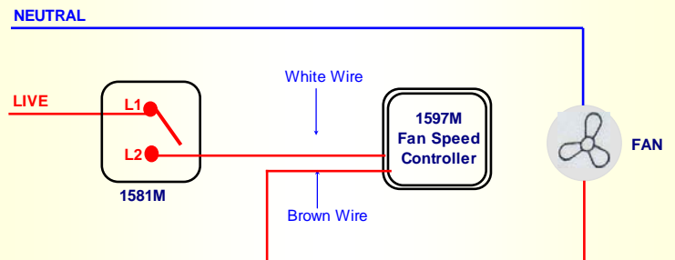
Cat 1597M Fan Speed Controller (1 Way Circuit)
