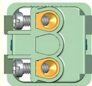
Rear view of 1515M, 1510MN 250V Indicator Switch Modules
